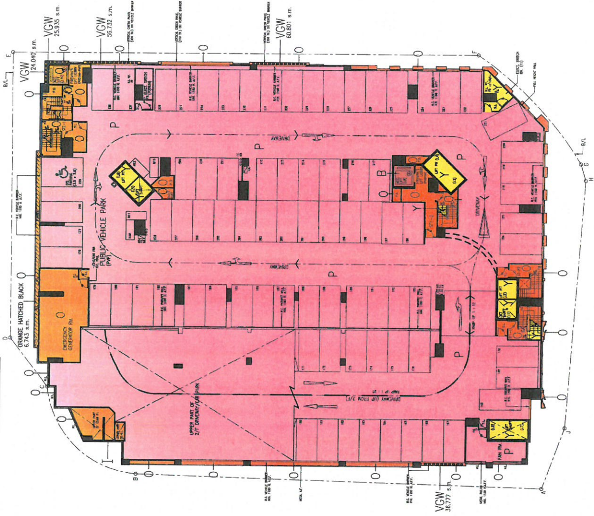
3RD FLOOR PLAN SCALE 1:300
