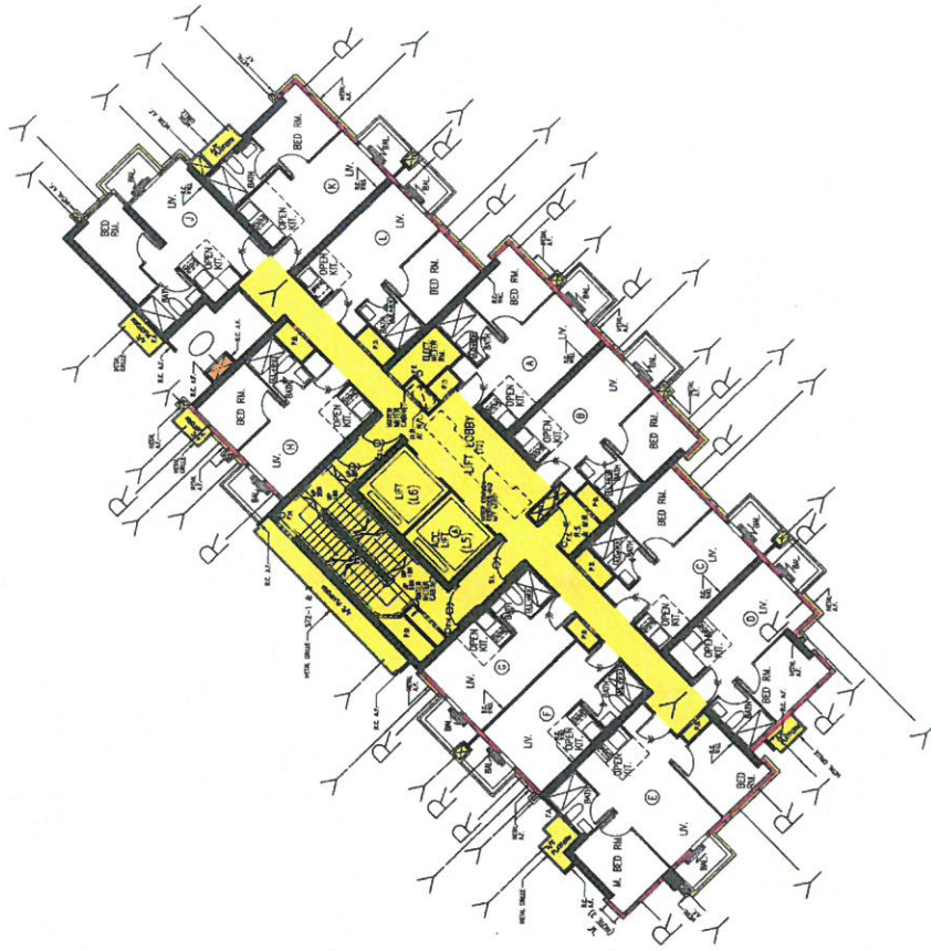
7TH - 31ST FLOOR PLAN (TOWER 2)
